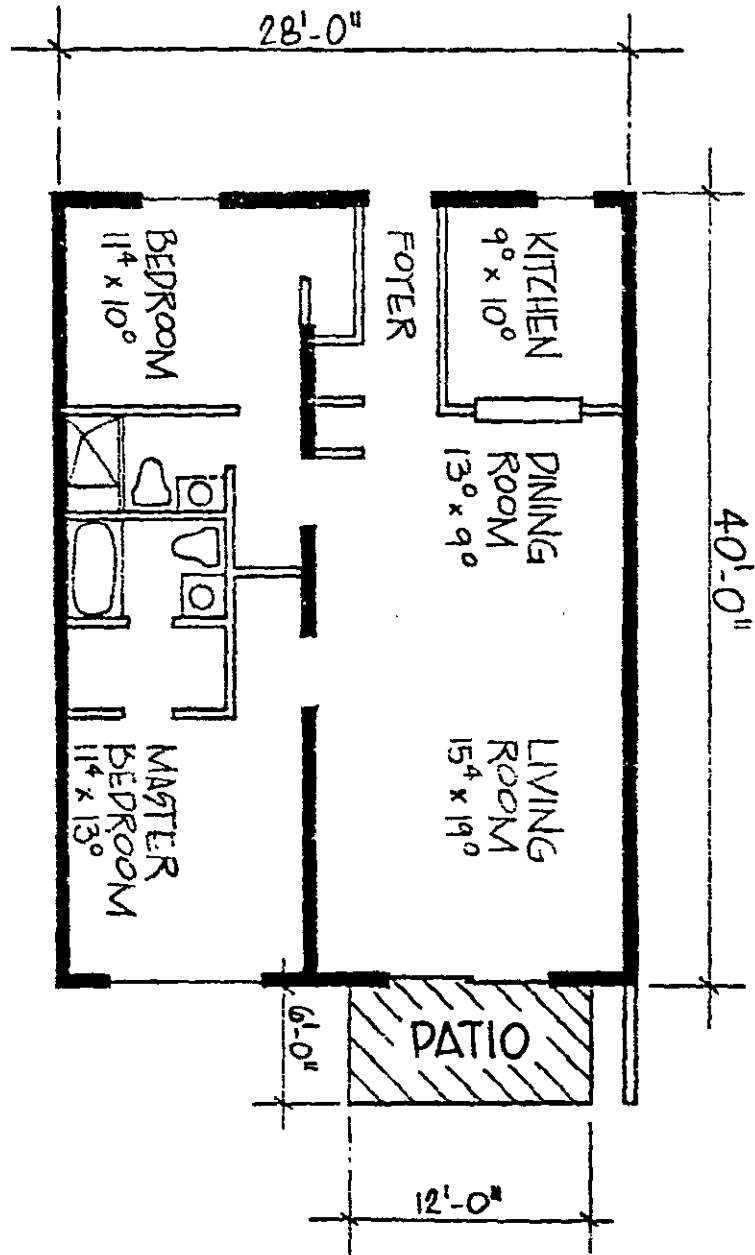
TYPICAL FLOOR PLAN UNIT B STANDARD - 1 STORY - 2 BEDROOM SCALE: 1/8" = 1'-0"
