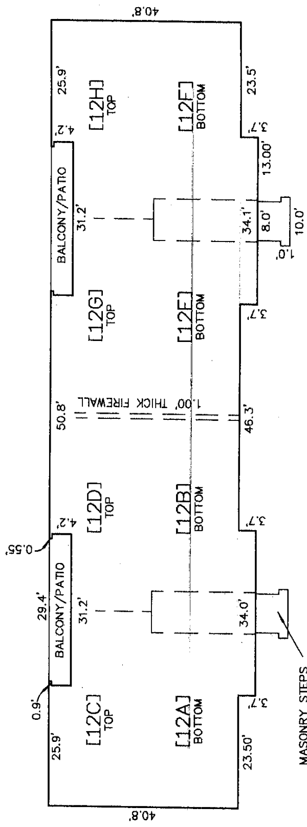
BUILDING NO. 12 FLOORPLAN 3 BEDROOM UNITS
